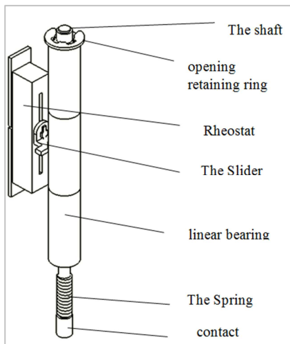
Figure 5. The displacement detector.
