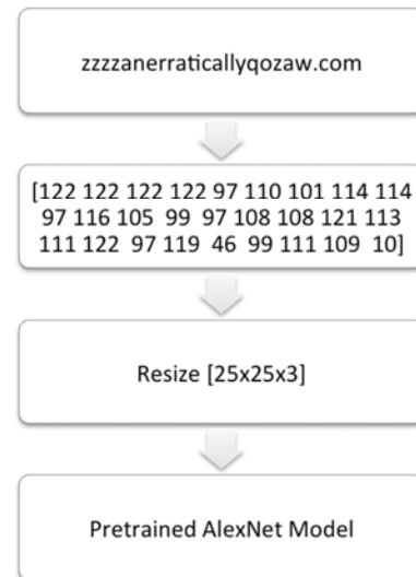
Figure 1. Process from raw input domain names called zzzanerraticallyqozaw.com to Alex Net models.
